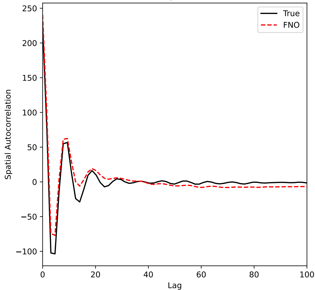
Autocorrelation Comparison with MSE = 48
