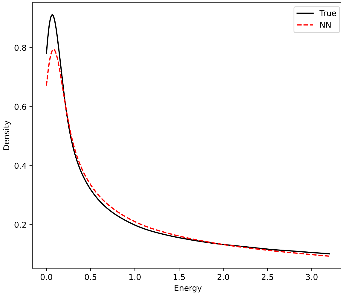
TKE Density Comparison with KS: 0.022, p-value: 0
