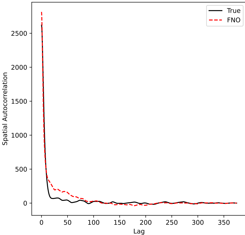
Autocorrelation Comparison with MSE = 3.7\text{e}+03
