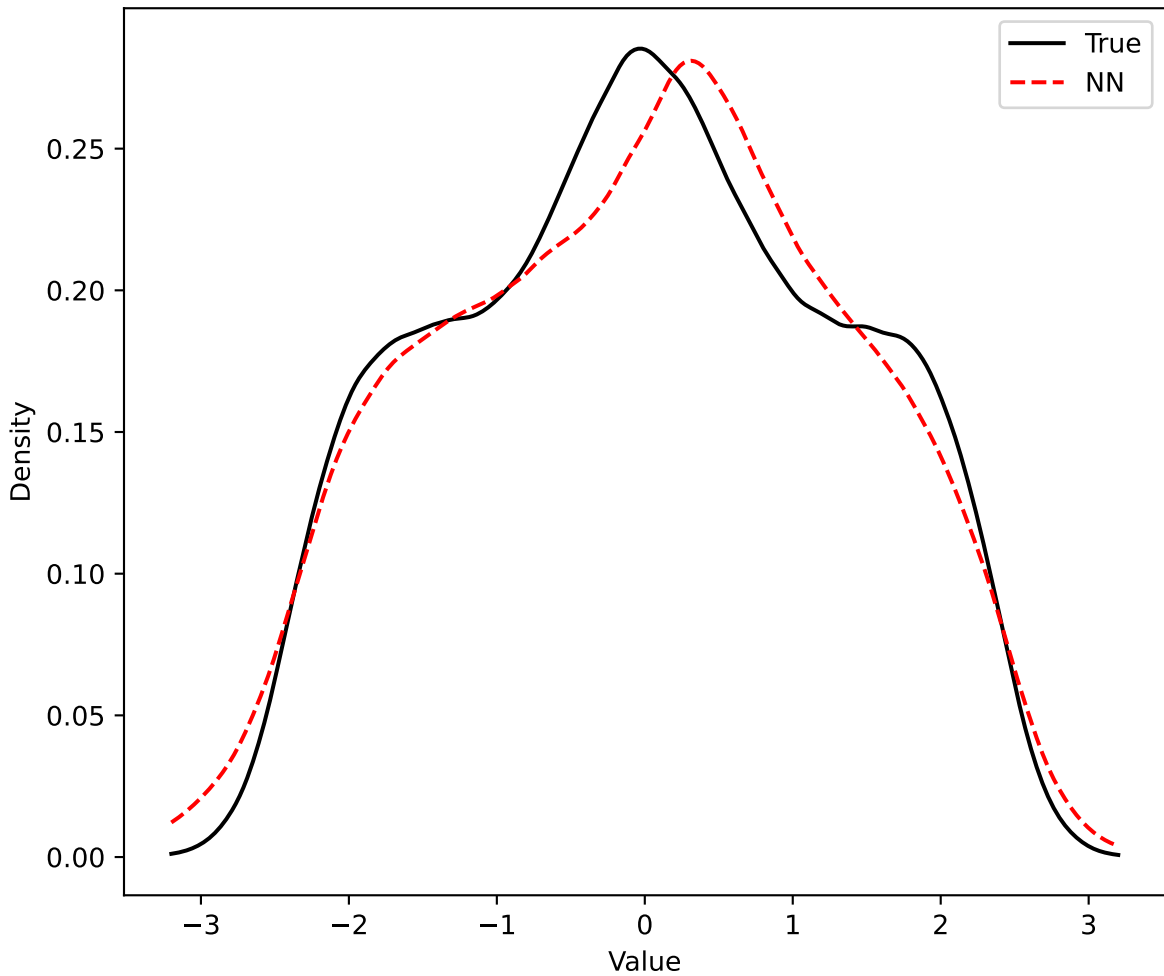
Empirical Density Comparison with KS: 0.016, p-value: 0
